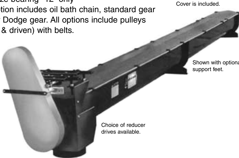
Shown with optional 90° spout.
